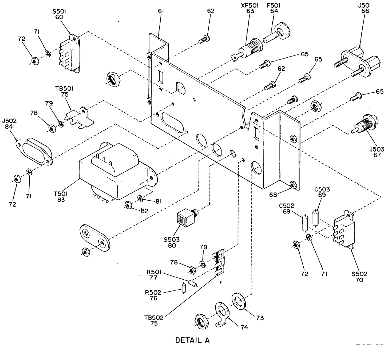
Figure 2. Indicator, Standing Wave Ratio IM-157E/U (Sheet 2 of 6).
