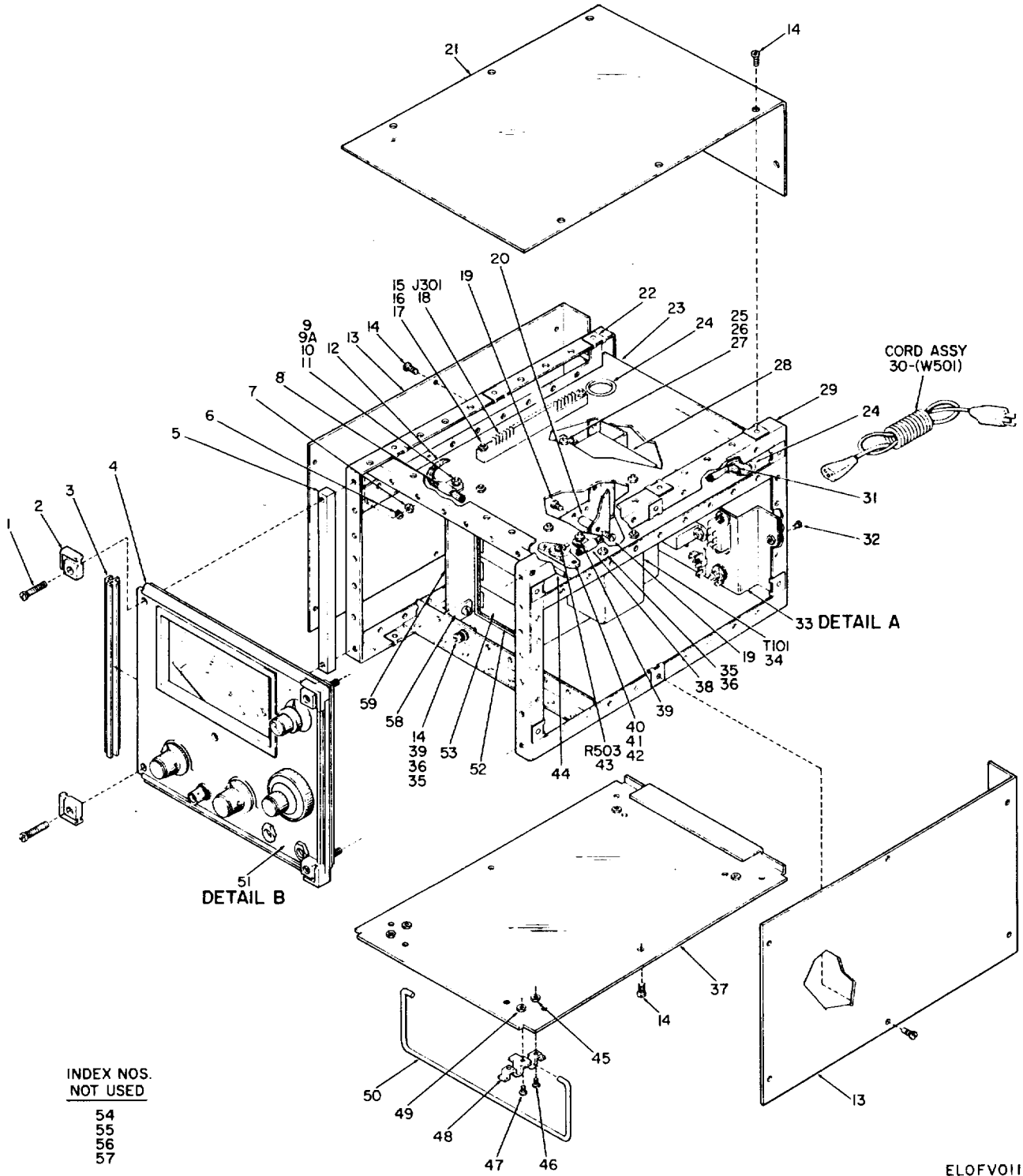
Figure 2. Indicator Standing Wave Ratio IM-157E/U (Sheet 1 of 6).
