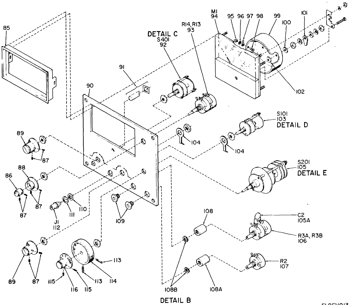
Figure 2. Indicator, Standing Wave Ratio IM-157E/U (Sheet 3 of 6).
