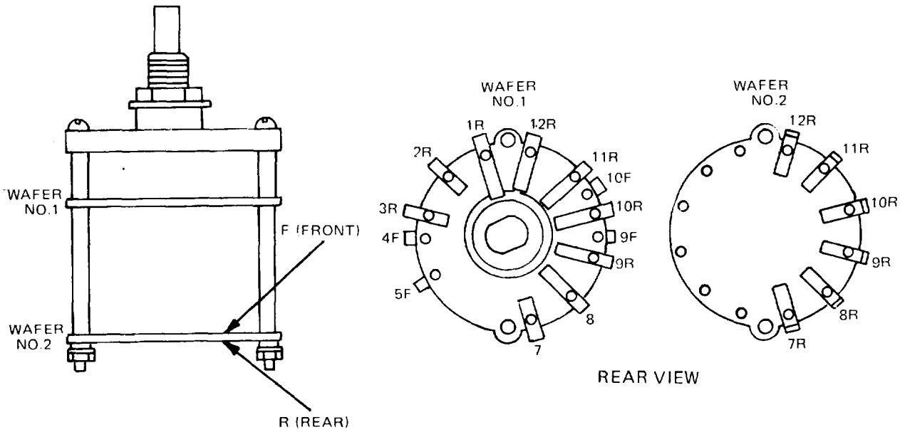
ITEMS NOT ILLUSTRATED IN INPUT SWITCH ASSEMBLY, S101
