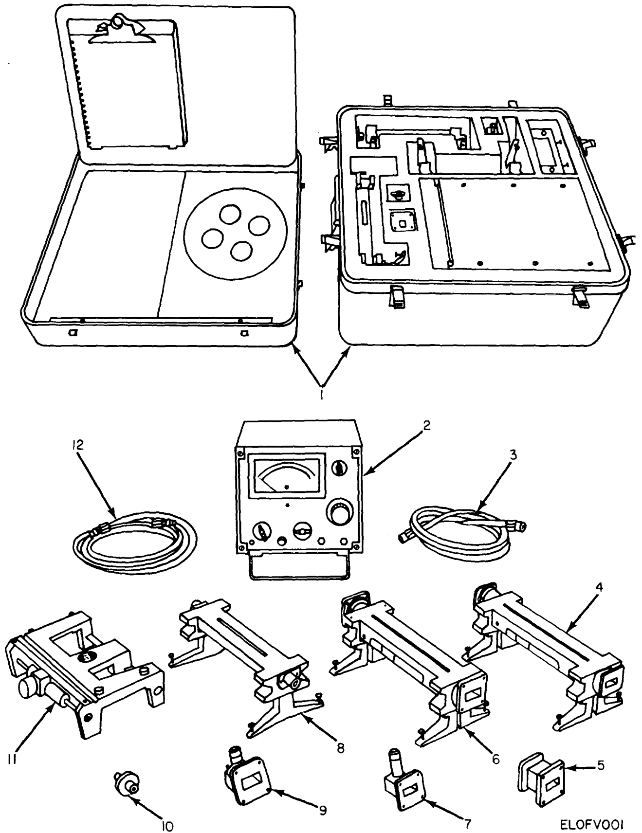
Figure 1. Measuring Set, Standing Wave Ratio AN/USM-37E.
