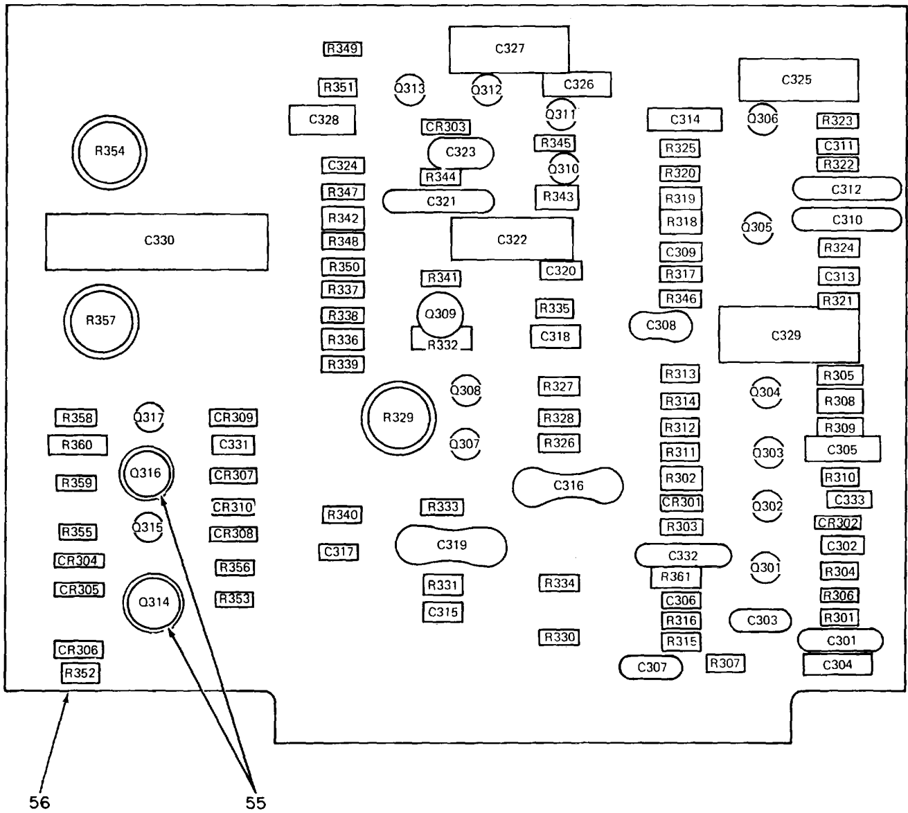
Figure 3. Indicator, Standing Wave Ratio IM-157E/U (Sheet 1 of 2).
